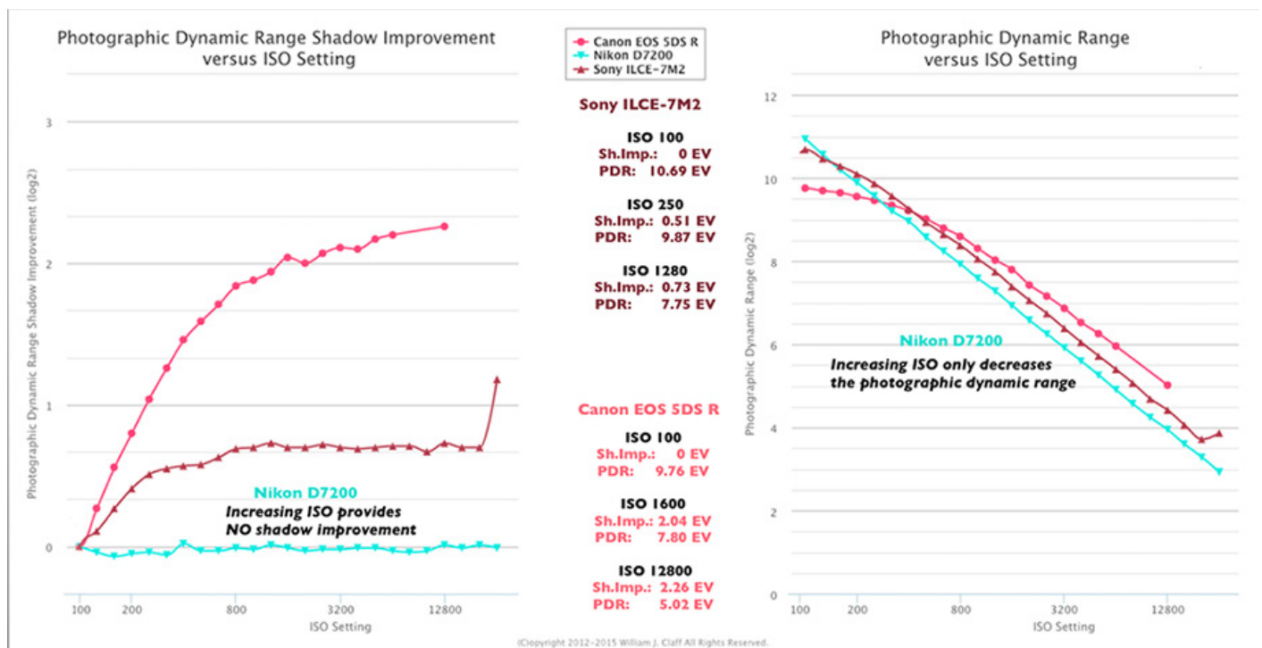
Figure 18. The correlation between ISO setting, Photographic Dynamic Range, and Shadow Improvement
