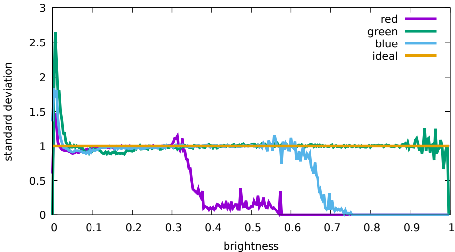
Flat noise levels - Hasselblad, L1D-20c, 100 ISO (DJI 0 750)
