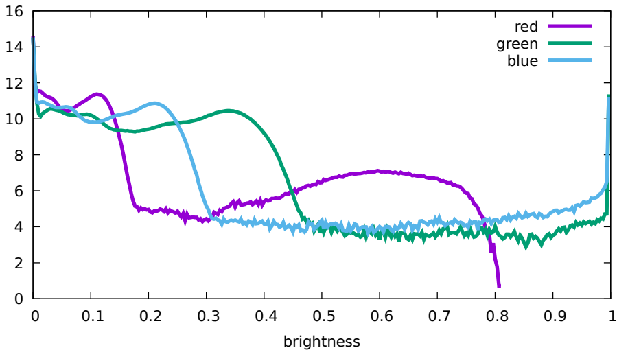
Flat histogram - Hasselblad, L1D-20c, 3200 ISO (DJI 0 756)
