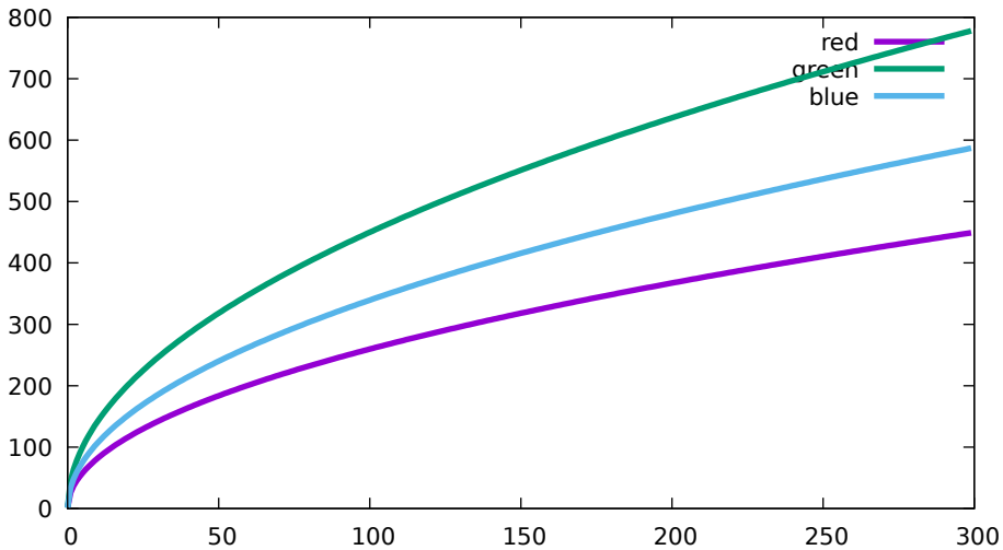
Conversion curves - Hasselblad, L1D-20c, 100 ISO (DJI 0 750)
