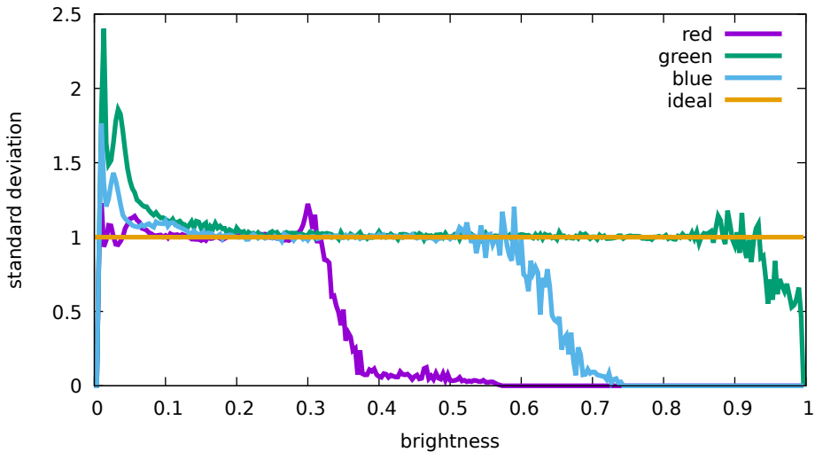
Flat noise levels - Hasselblad, L1D-20c, 1600 ISO (DJI 0 755)
