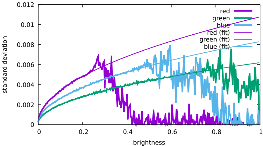
Noise levels - Hasselblad, L1D-20c, 800 ISO (DJI 0 754)
