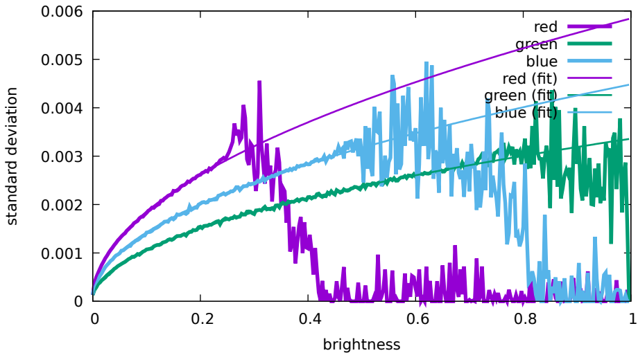
Noise levels - Hasselblad, L1D-20c, 200 ISO (DJI 0 751)
