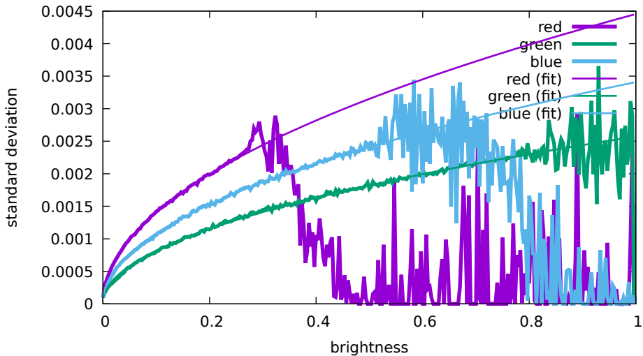
Noise levels - Hasselblad, L1D-20c, 100 ISO (DJI 0 750)
