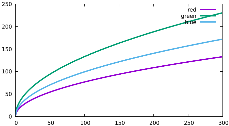
Conversion curves - Hasselblad, L1D-20c, 1600 ISO (DJI 0 755)
