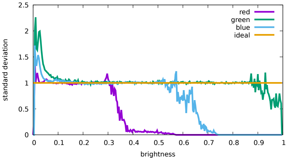
Flat noise levels - Hasselblad, L1D-20c, 800 ISO (DJI 0 754)
