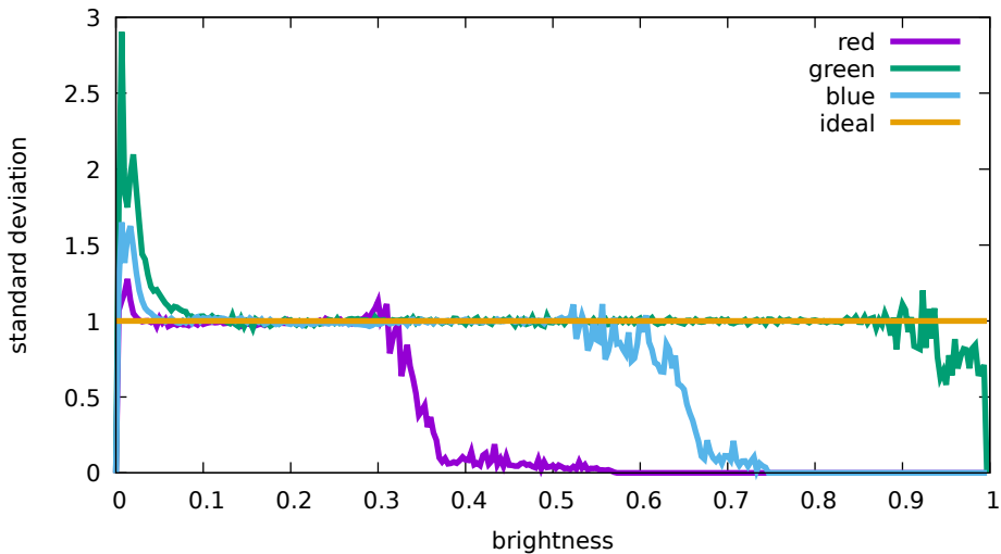
Flat noise levels - Hasselblad, L1D-20c, 400 ISO (DJI 0 752)
