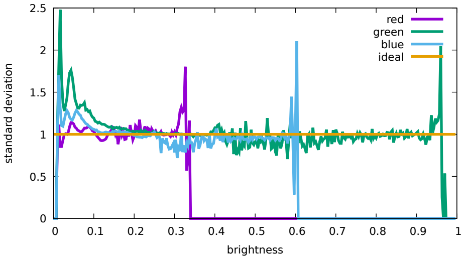
Flat noise levels - Hasselblad, L1D-20c, 12800 ISO (DJI 0 758)
