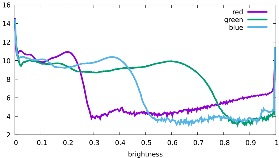
Flat histogram - Hasselblad, L1D-20c, 800 ISO (DJI 0 754)
