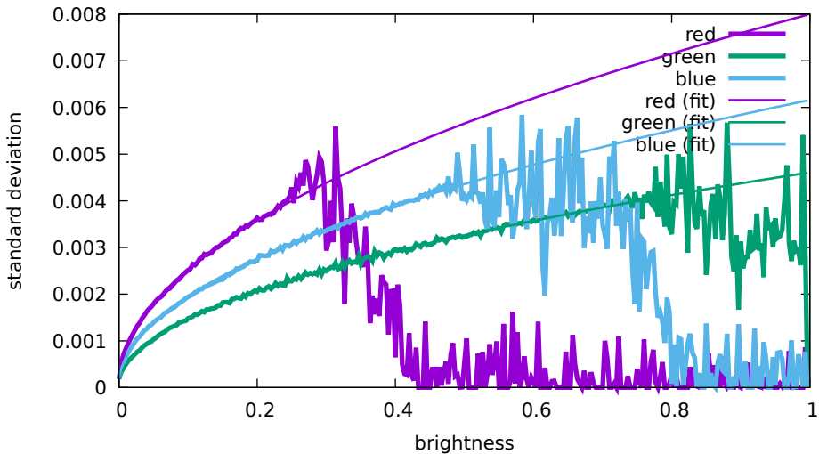
Noise levels - Hasselblad, L1D-20c, 400 ISO (DJI 0 752)
