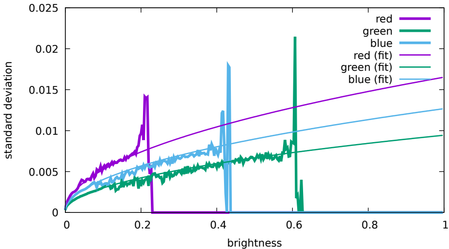
Noise levels - Hasselblad, L1D-20c, 12800 ISO (DJI 0 758)
