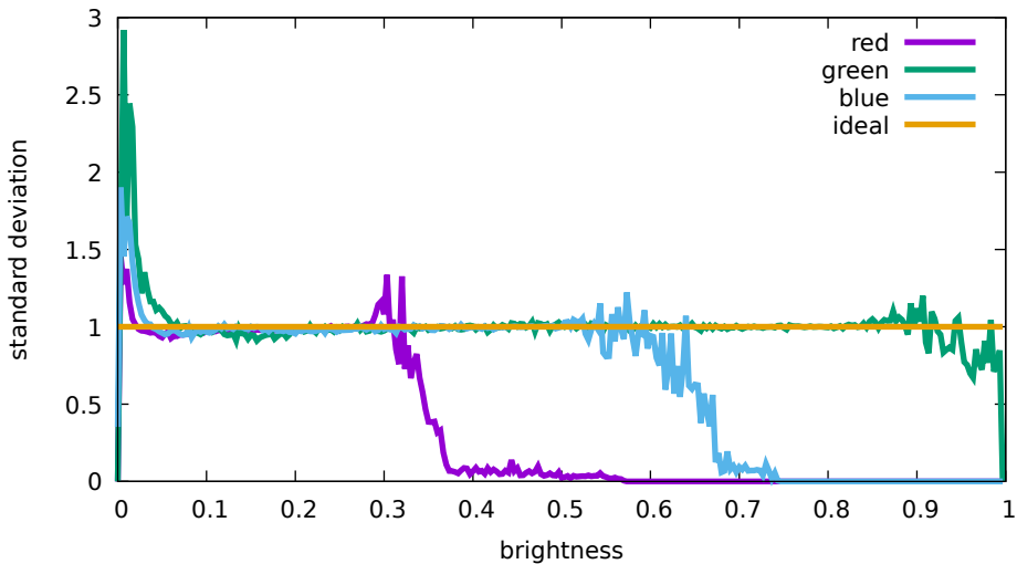
Flat noise levels - Hasselblad, L1D-20c, 200 ISO (DJI 0 751)
