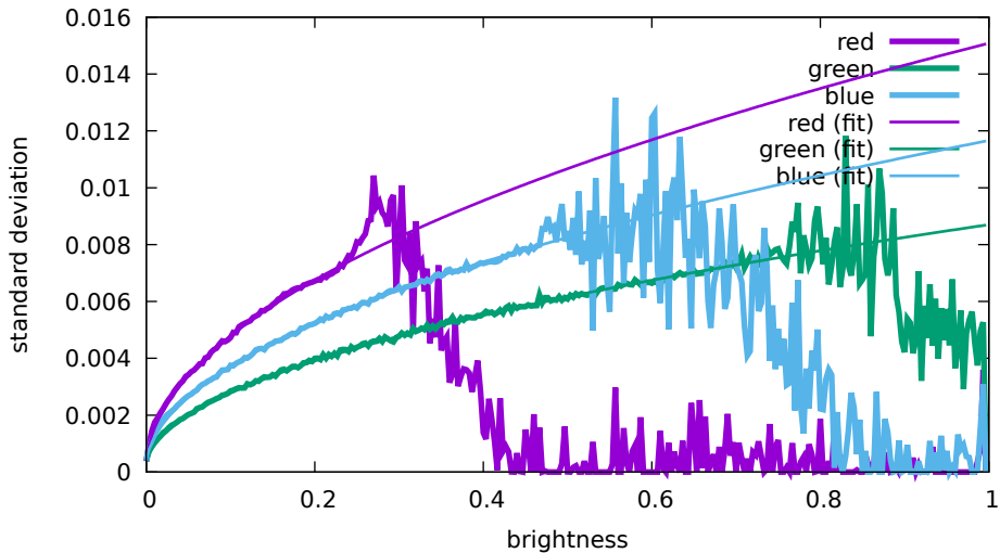
Noise levels - Hasselblad, L1D-20c, 1600 ISO (DJI 0 755)
