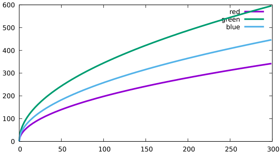
Conversion curves - Hasselblad, L1D-20c, 200 ISO (DJI 0 751)
