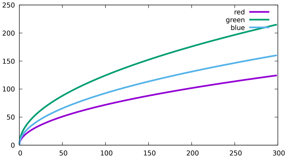
Conversion curves - Hasselblad, L1D-20c, 3200 ISO (DJI 0 756)
