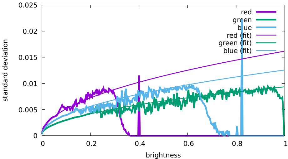
Noise levels - Hasselblad, L1D-20c, 6400 ISO (DJI 0 757)
