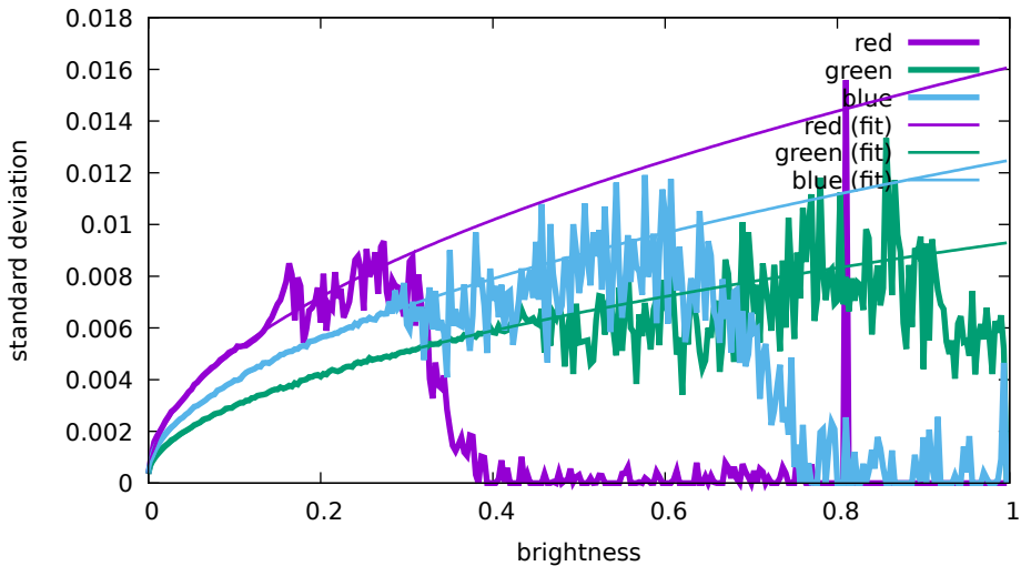
Noise levels - Hasselblad, L1D-20c, 3200 ISO (DJI 0 756)
