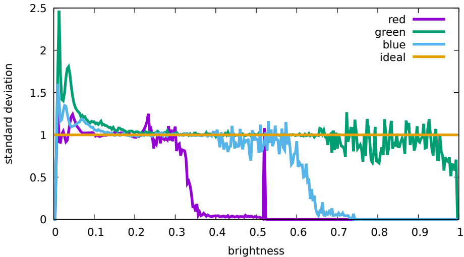
Flat noise levels - Hasselblad, L1D-20c, 3200 ISO (DJI 0 756)
