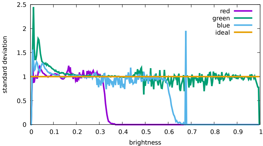
Flat noise levels - Hasselblad, L1D-20c, 6400 ISO (DJI 0 757)
