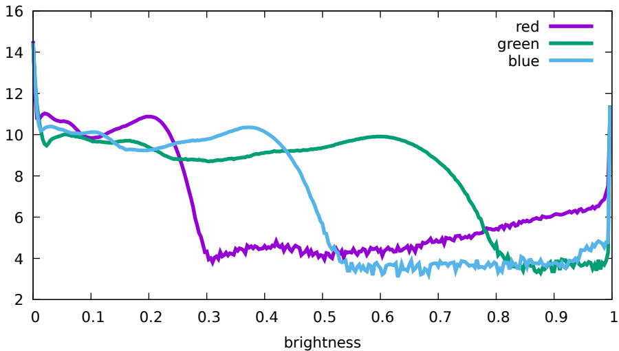
Flat histogram - Hasselblad, L1D-20c, 1600 ISO (DJI 0 755)
