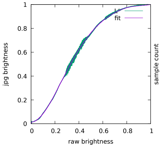
spline fit
